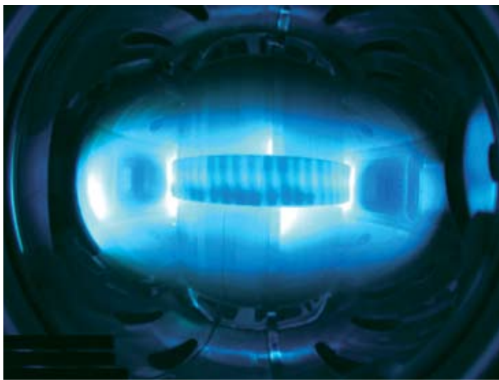
A magnetically confined plasma in KSTAR. The ultra-hot plasma radiates in a spectrum that cannot be seen by the human eye. Visible in this image are the colder regions on the outer edge of the plasma.
