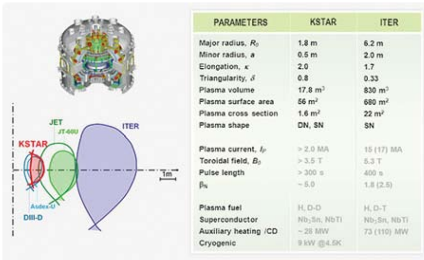
Figure 3 KSTAR AND ITER PARAMETERS COMPARED
