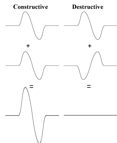
Constructive interference: The two waves add to produce a larger wave. Destructive interference: The two waves are each other's negative, and thus add up to zero wave.
